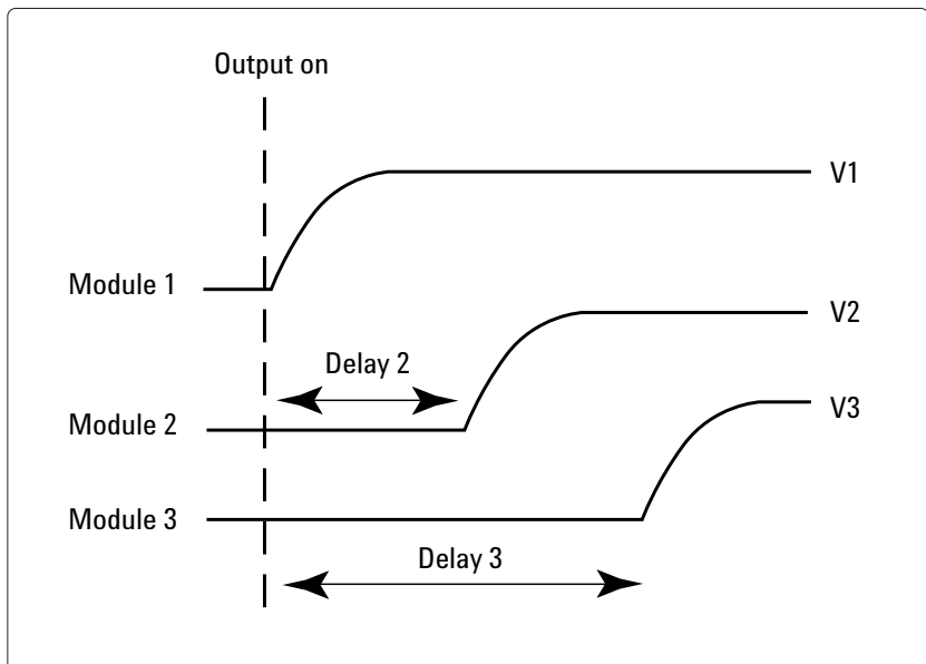
Figure 2. Output Sequencing
